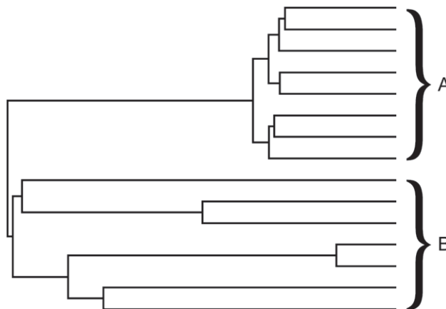
FIGURE 1. A motivating example showing “bursting” diversification. Namely, in the oldest part of the tree, diversification events happen exclusively in the B lineage, followed by a period of high diversification rate in the A lineage. This paper constructs a statistical framework for analyzing such “bursting” patterns or their opposite.
